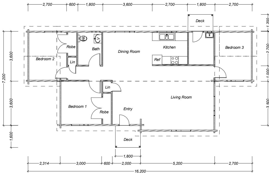
Floorplan
