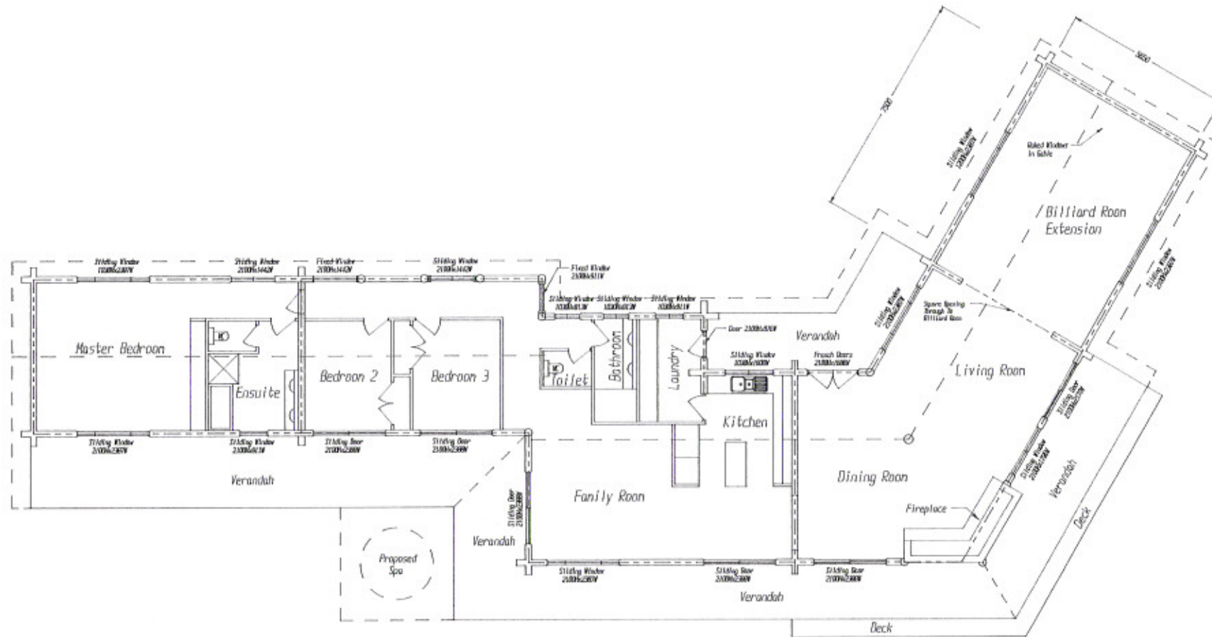
Floor Plan (Scale 1:125)
