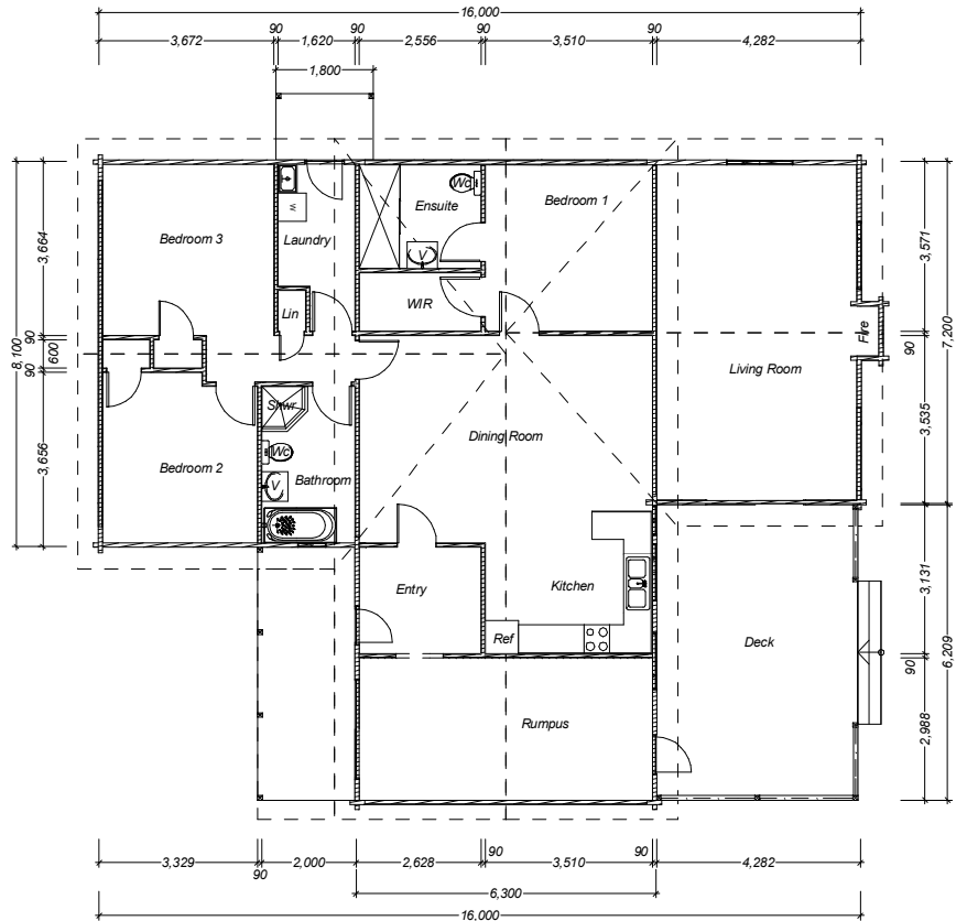
Floorplan
