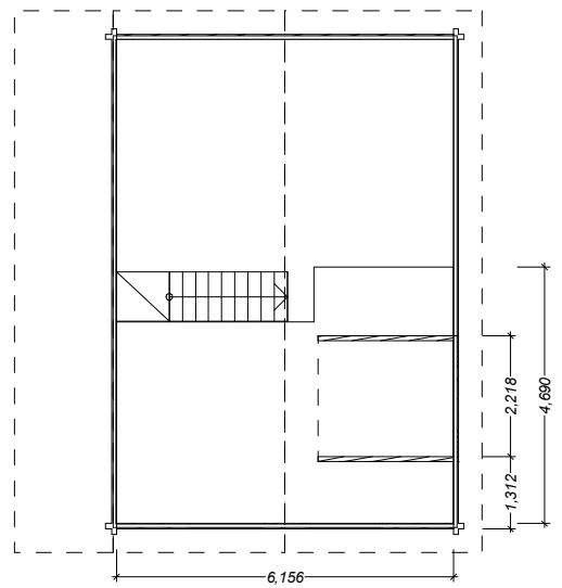
Upper Floor
