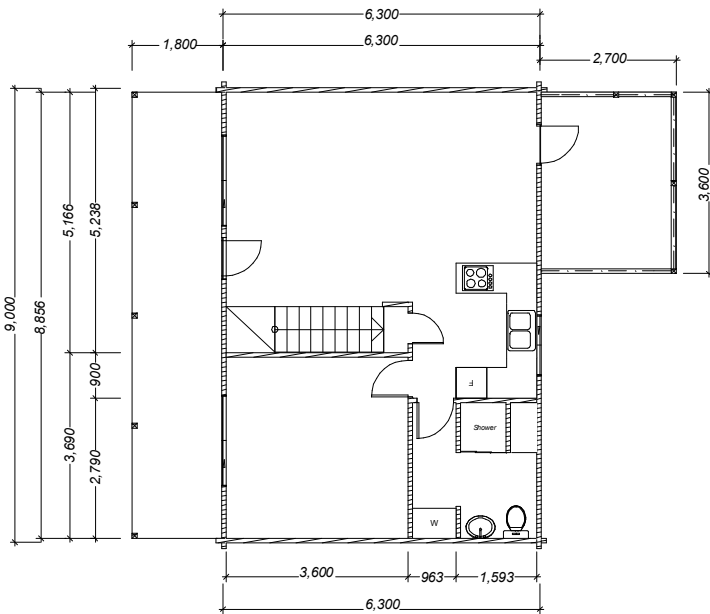
Lower Floor
