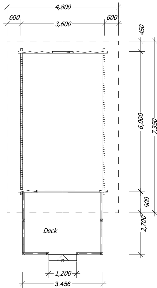
Floorplan
