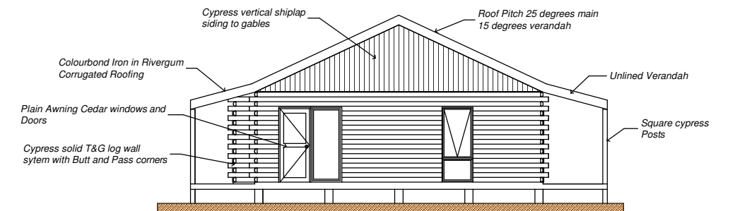
Elevation 1 - Scale 1:150
