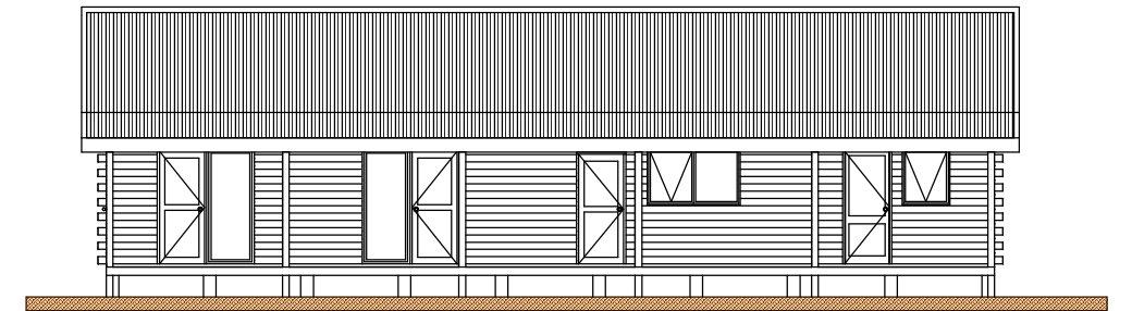
Elevation 4 - Scale 1:150
