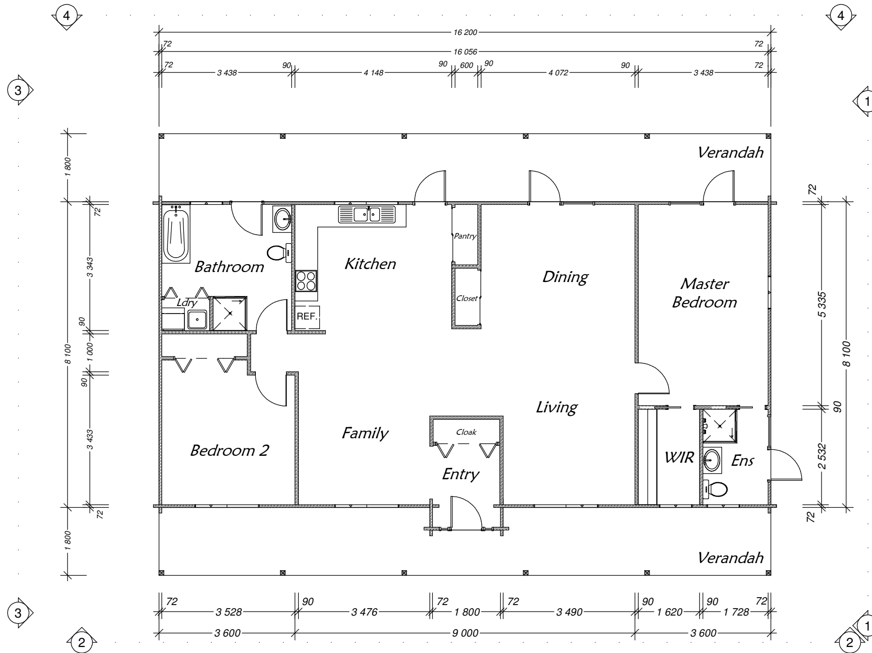
Floorplan - Scale 1:100
