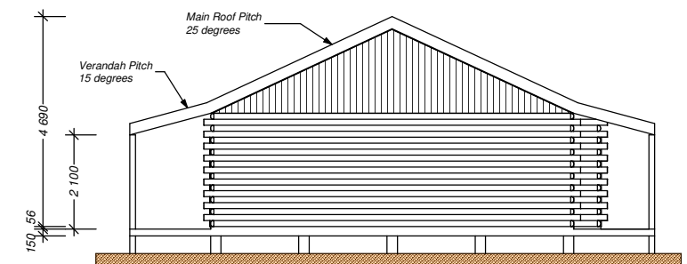
Elevation 3 - Scale 1:150
