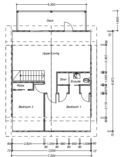
Floorplan Upper
