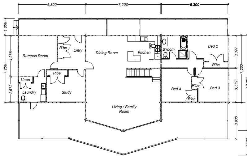
Lower Floor
