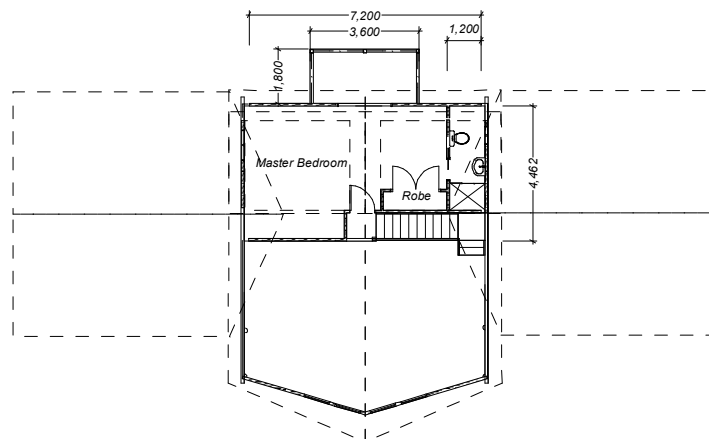
Upper Floor
