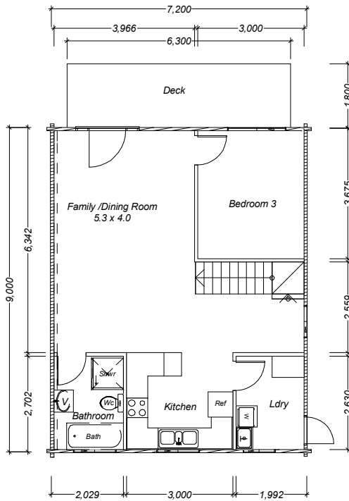
Lower Floor
